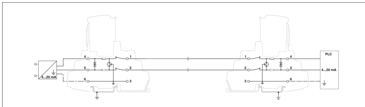
Fig. 82: Example of a measuring signal transmission (4...20 mA) with surge protection
